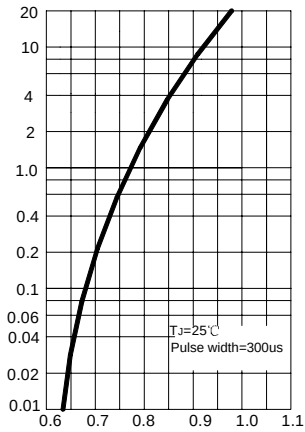
FIG.2 -- TYPICAL FORWARD CHARACTERISTICS
