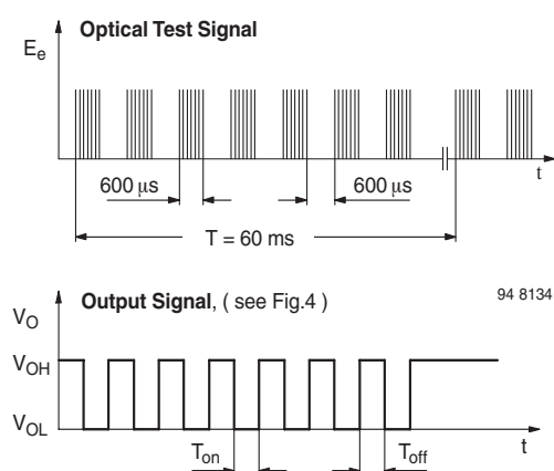
Figure 3. Output Function
