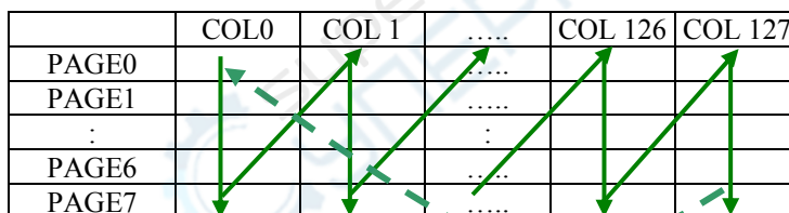
Figure 10-4 : Address Pointer Movement of Vertical addressing mode
