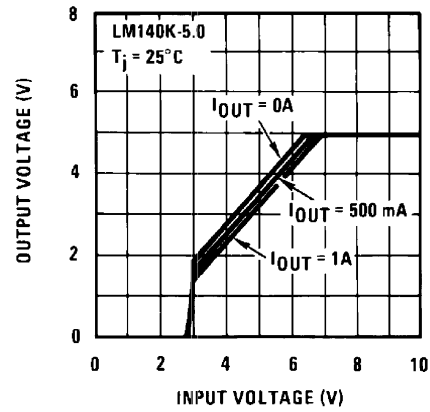
Dropout Characteristics
