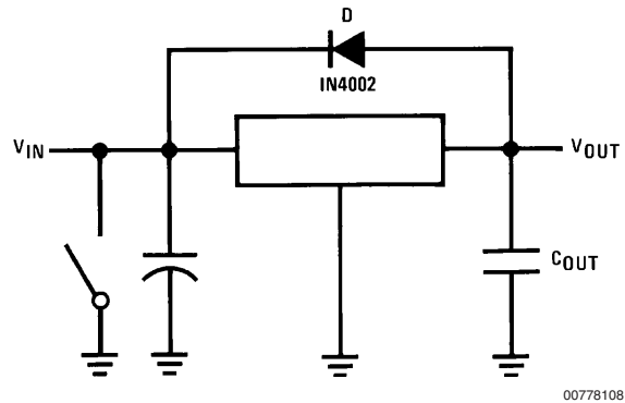
FIGURE 1. Input Short
