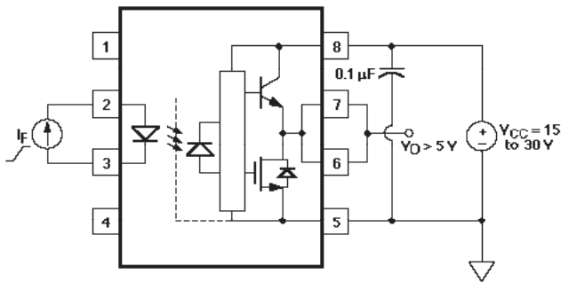
Figure 21. I_{FL} Test Circuit.
