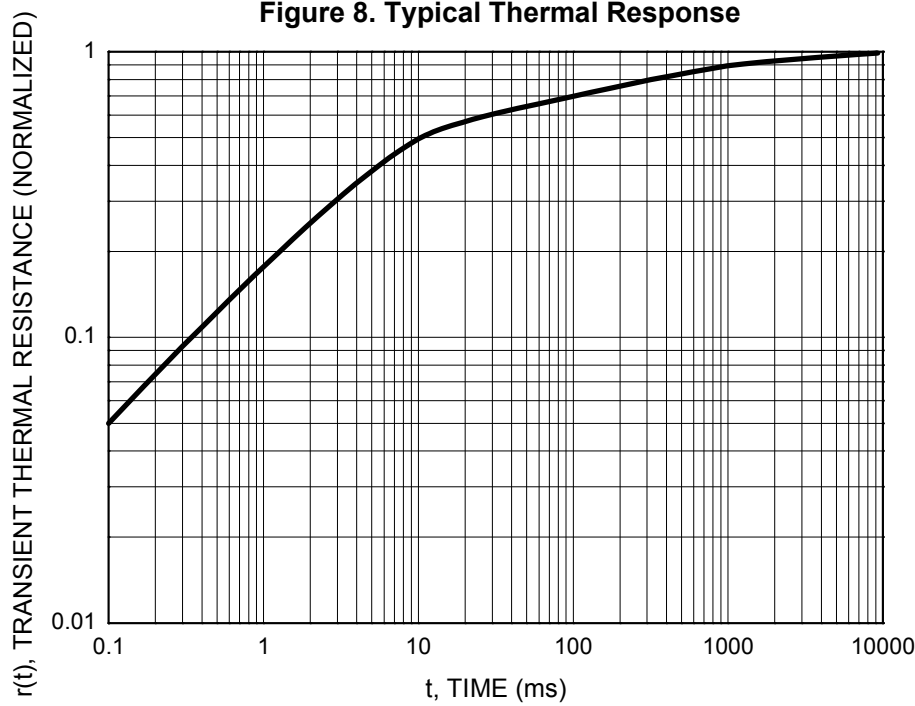
Figure 8. Typical Thermal Response
