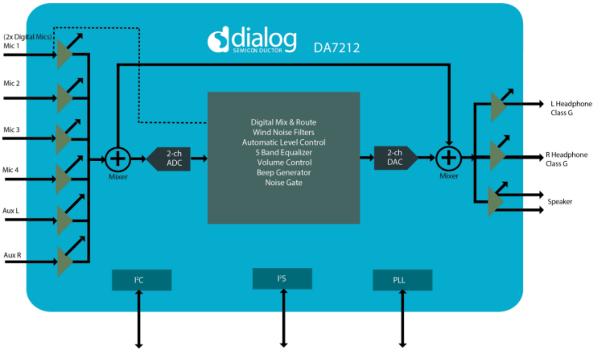
Figure 1: Component values shown for a typical application
