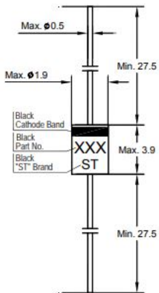
Glass Case DO-35
