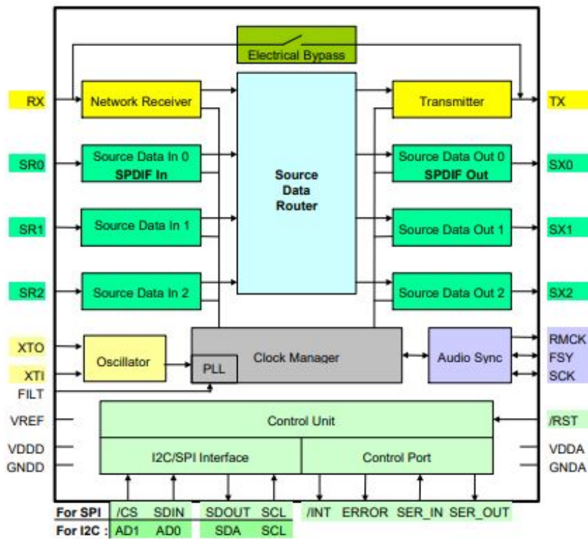
Block Diagram
