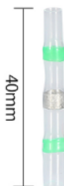
S41 0.75~1.5mm 2
